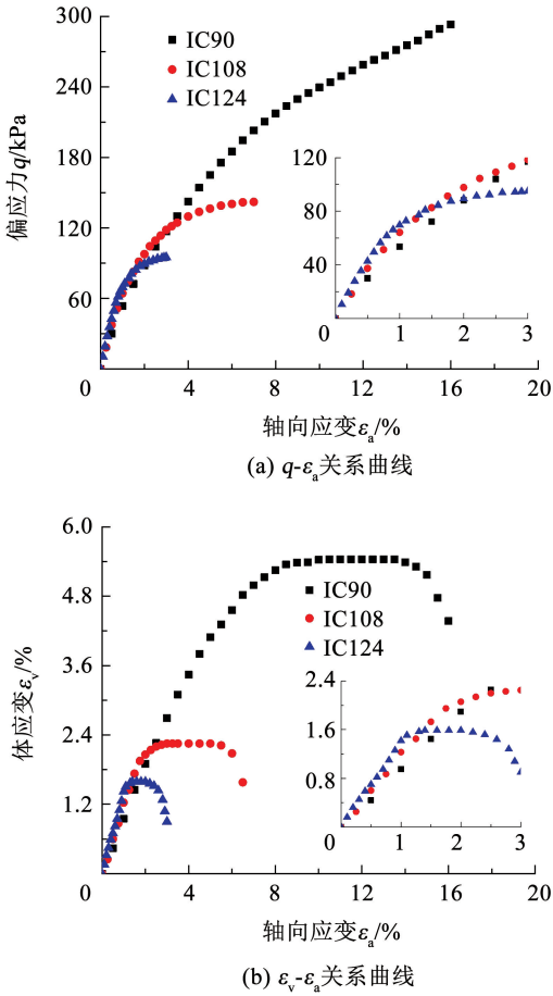
图4 \Delta\sigma_3 < 0 的压缩路径下垃圾土的应力-应变关系 Fig. 4 Stress-strain relationship of MSW under compression stress path tests with \Delta\sigma_3 < 0
