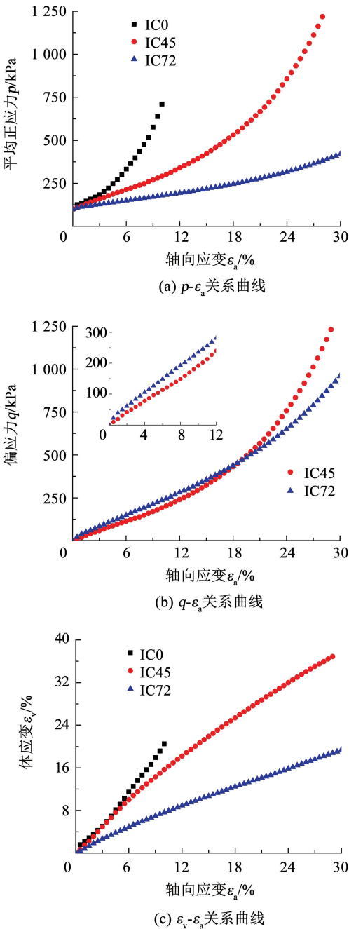
图3 \Delta\sigma_3 \geq 0 的压缩路径下垃圾土的应力-应变关系 Fig. 3 Stress-strain relationship of MSW under compression stress path tests with \Delta\sigma_3 \geq 0
